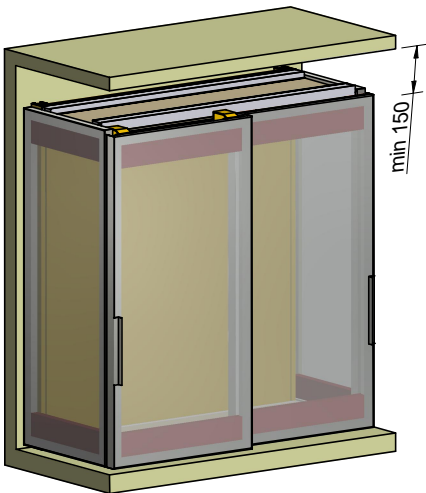
2.2 One side wall, other frame
