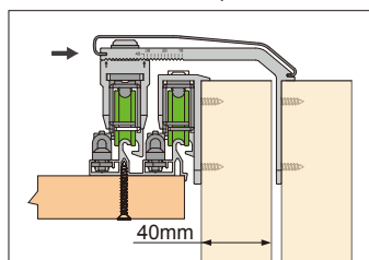
40mm Door panel
