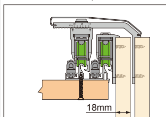
18mm Door panel
